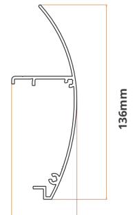
10. Radiused Gutter Fascia
