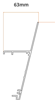
11. Angled Gutter Fascia
