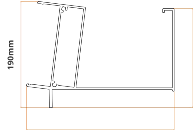
3. Standard Gutter
