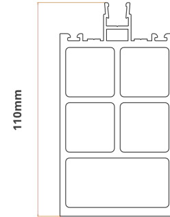
8. Heavy Duty Intermediate Roof Beam
