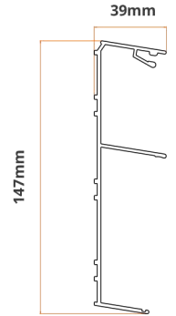
5. Wall Plate
