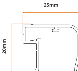
13. Nosing For Polycarbonate
