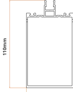
2. Heavy Duty Post
